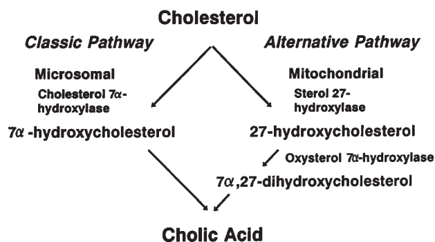
Figure 1 Flow diagram illustrating two pathways for bile acid synthesis. Cholesterol serves as the sole substrate and is converted to cholic acid via both classic and alternative pathways. Microsomal cholesterol 7 \alpha -hydroxylase is the initial and rate-controlling enzyme for the classic pathway, whereas mitochondrial sterol 27-hydroxylase initiates the alternative pathway and might be rate limiting. The product, 27-hydroxycholesterol, is then 7 \alpha -hydroxylated by microsomal oxysterol 7 \alpha -hydroxylase (27-hydroxycholesterol-7 \alpha -hydroxylase), which is different from microsomal cholesterol 7 \alpha -hydroxylase.
